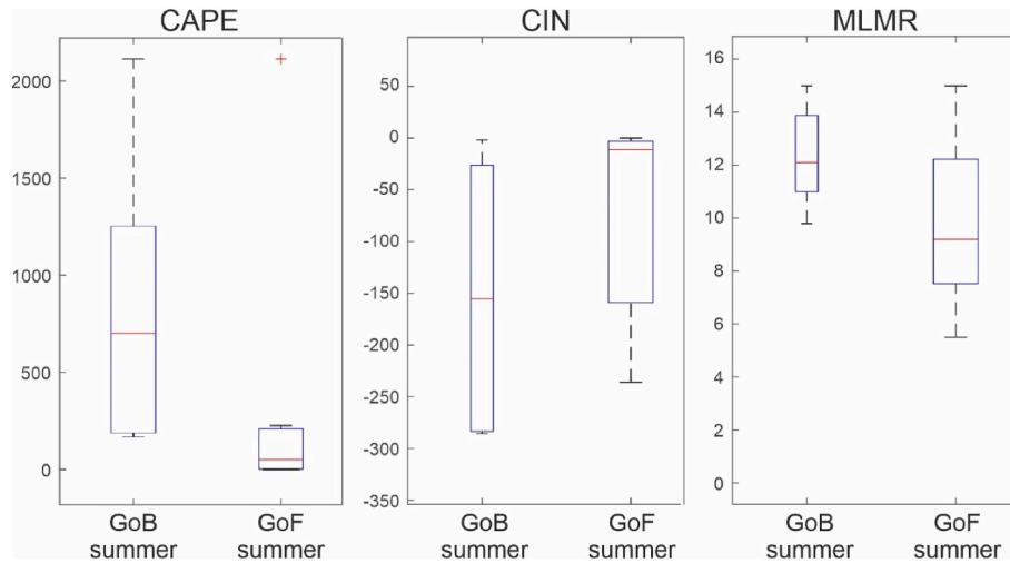
Fig. 10. Box-plot distribution of CAPE ( \text{J kg}^{-1} ), CIN ( \text{J kg}^{-1} ) and MLMR ( \text{g kg}^{-1} ) during summer-type events in the Gulf of Bothnia (GoB) and Gulf of Finland (GoF). Central red lines stand for median values, bottom and top of boxes for 25 and 75 percentile values and top and bottom of whiskers for minima and maxima; red crosses stand for outliers.
