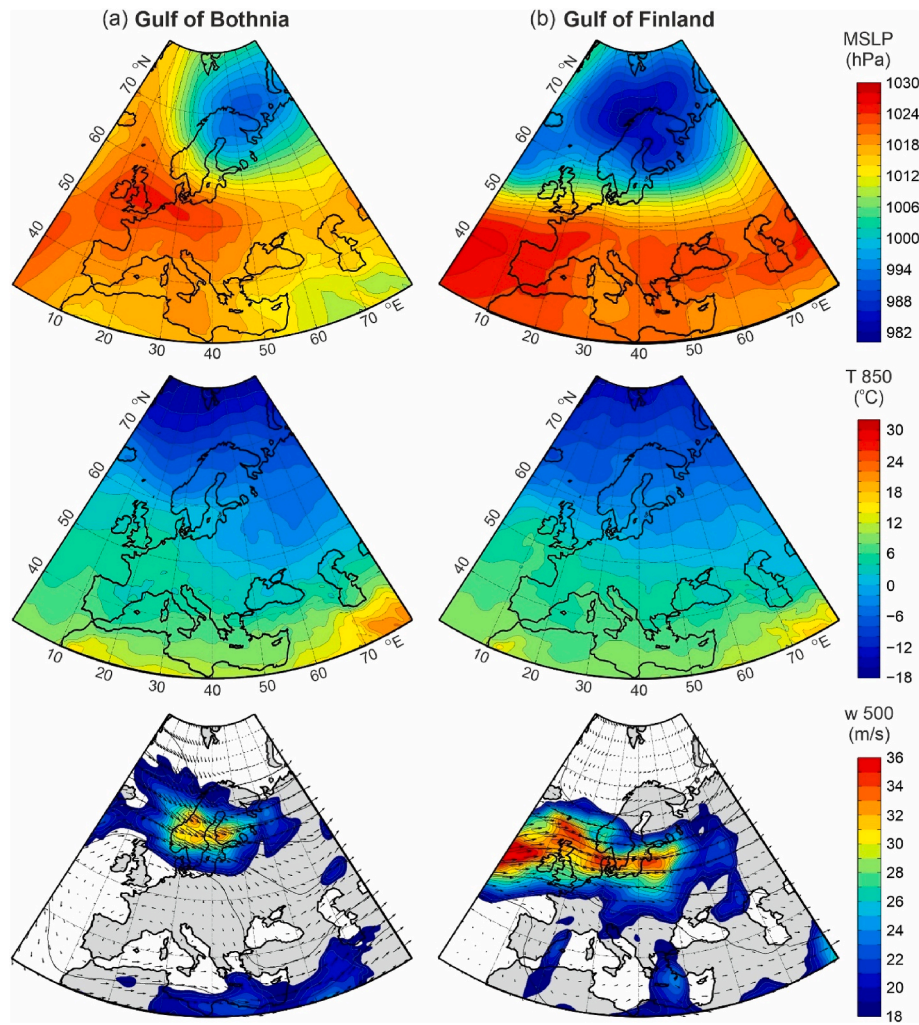
Fig. 11. Mean sea level pressure (top), temperature at 850 hPa (middle) and geopotential and winds at 500 hPa (bottom) over Europe during the winter-type sea level events over: (a) the Gulf of Bothnia and (b) Gulf of Finland. Only winds faster than 18 \text{ m s}^{-1} are coloured in the bottom plot.
