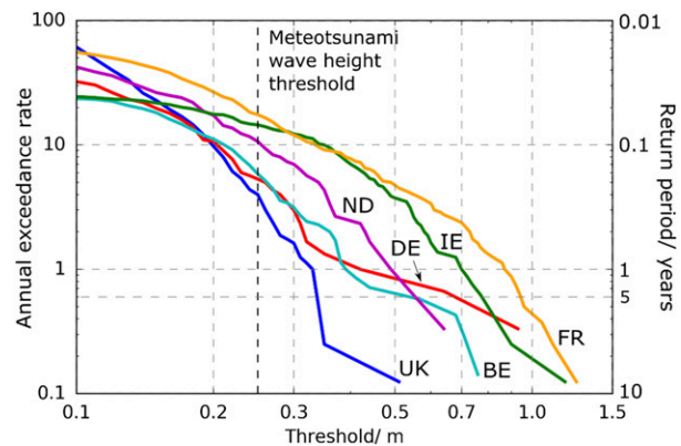
FIG. 3. NSLOTT annual size-exceedance rate for thresholds between 0.1 and 1.5 m from tide gauges grouped across each country. IE/Republic of Ireland, green; UK/United Kingdom, blue; FR/France, orange; BE/Belgium, cyan; ND/The Netherlands, purple; DE/Germany, red. The dashed black vertical line is at 0.25 m, which is the meteotsunami wave-height threshold. Return period in years is shown on the right-hand vertical axis. A return period of n years indicates that on average, one NSLOTT exceeds the threshold every n years.
