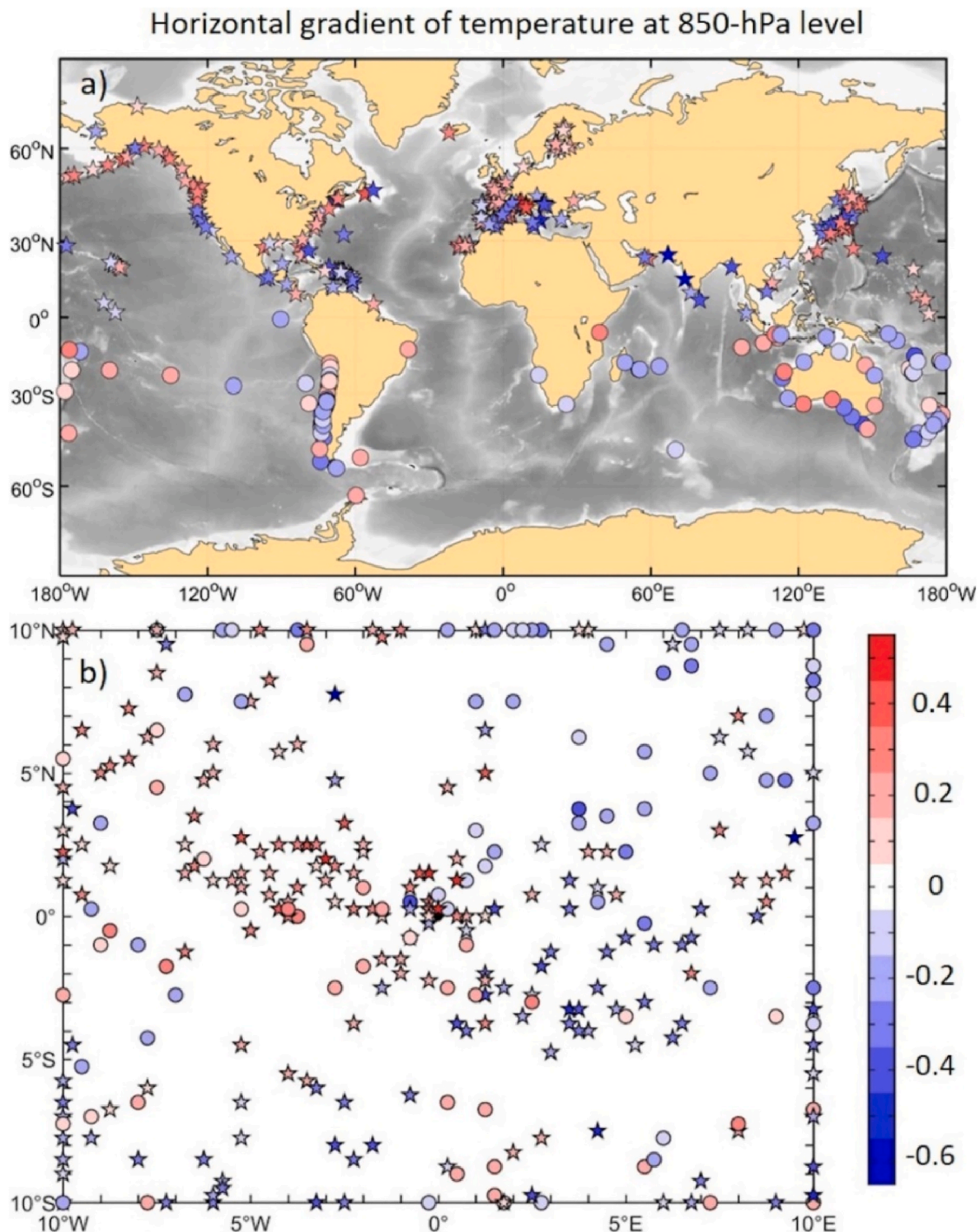
Fig. 8. As in Fig. 5, but for horizontal gradient of temperature at 850-hPa level.
